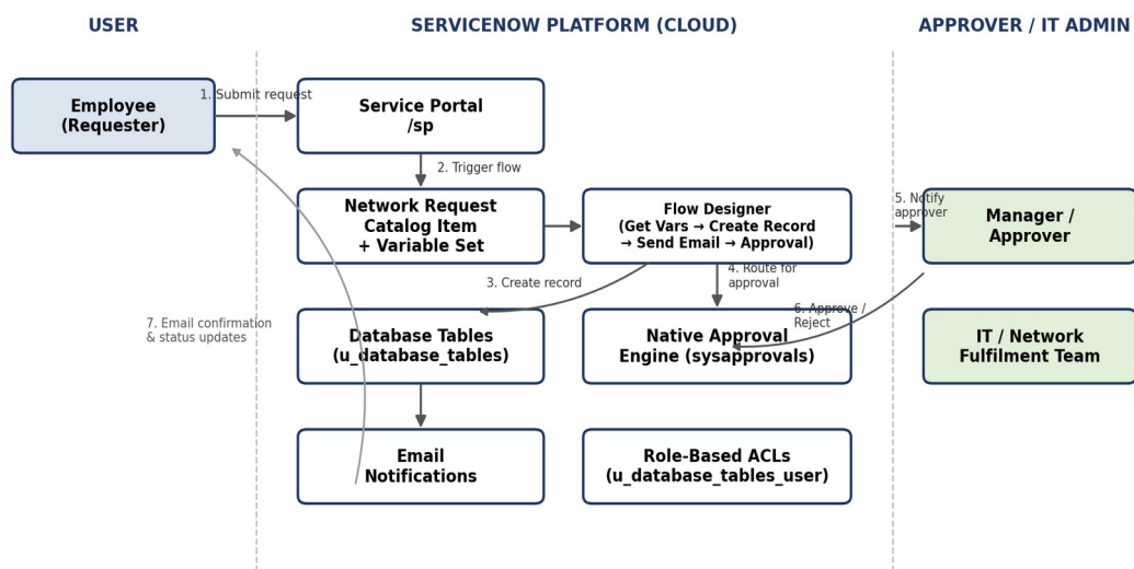
Figure 1: Architecture and data flow of the Automated Network Request Management solution on ServiceNow
